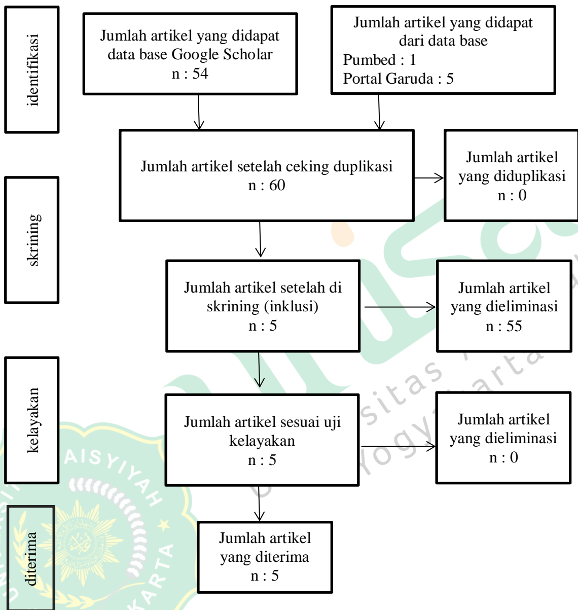
Diagram PRISMA
