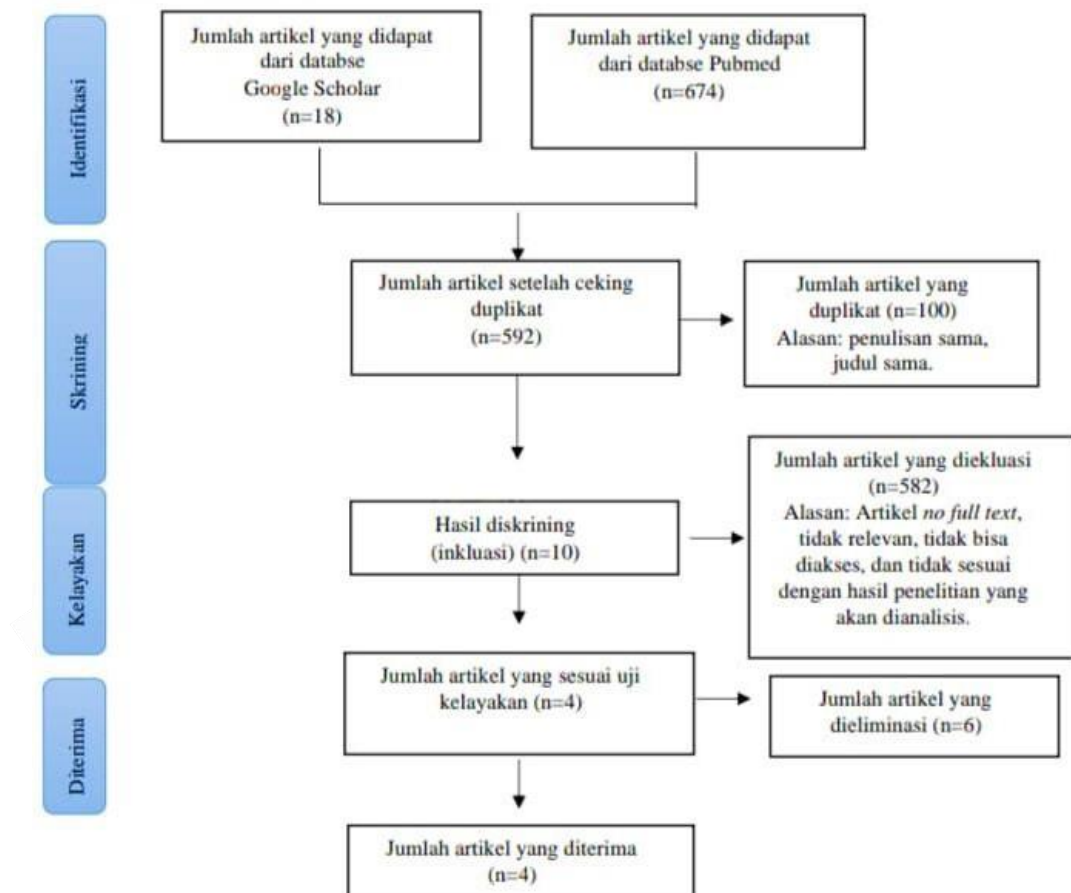
Gambar 1. Diagram PRISMA
